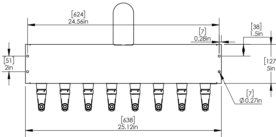
Top View
